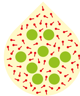
Solubilized preparation
