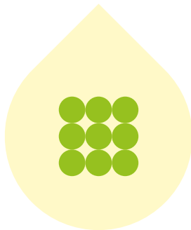
Conventional preparation
